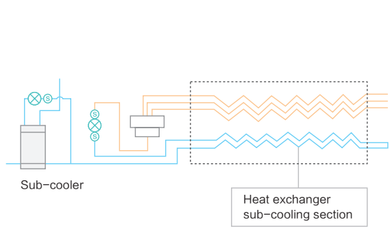
Two-stage sub-cooling cycle diagram
