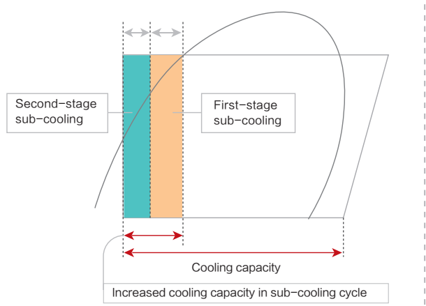
Two-stage sub-cooling pressure enthalpy diagram
